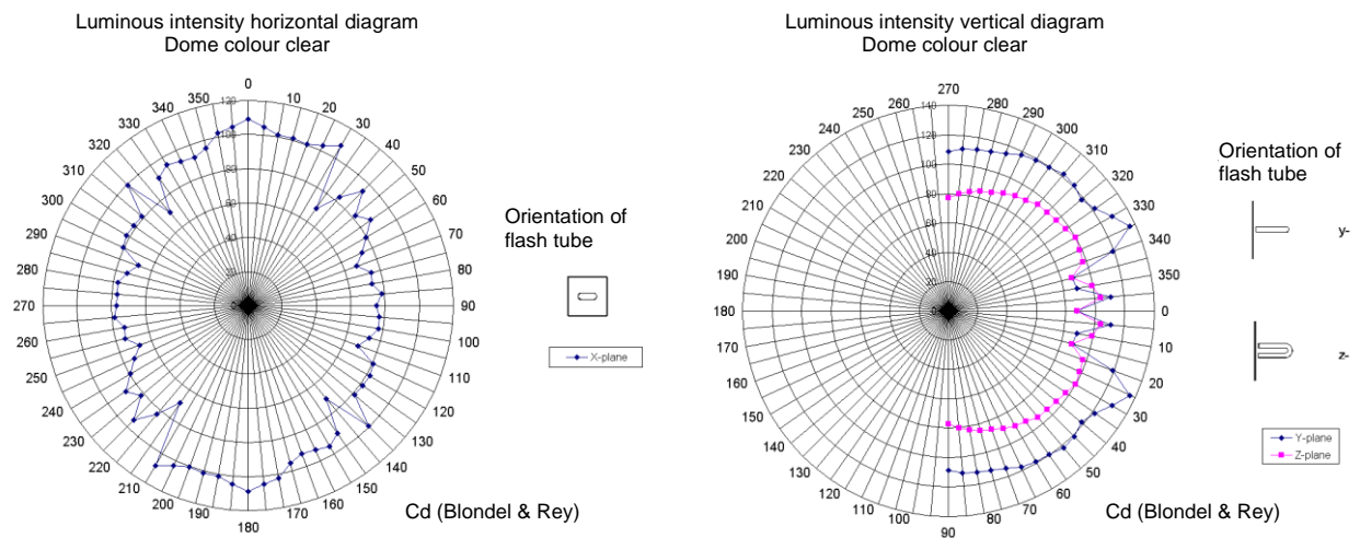
Fig. 5 Directional diagrams
