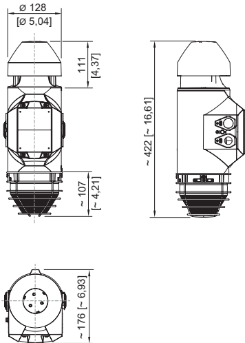
YL60/3 omnidirectional horn
